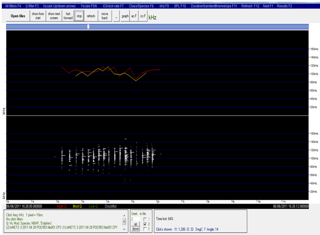
Figure 3.4: Screen grab of C-POD.exe, showing a harbour porpoise click train ((i) porpoise-like, but other categories include (ii) dolphins, (iii) other train sources, (iv) unclassified, (v) boat sonars)
