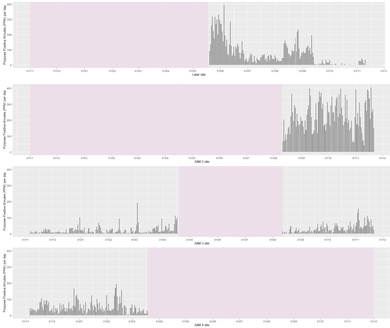
Figure 4.4-4.7: Number of Harbour Porpoise positive detections minutes (PPM) per day recorded across all locations (Lidar, SAM2, SAM3 and SAM4).
